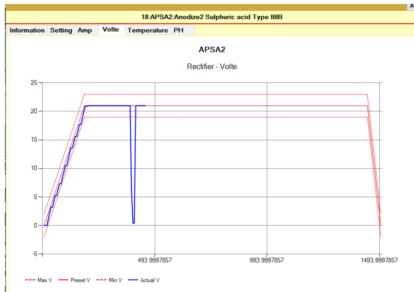
Fig.6 Rectifier Output Graph
